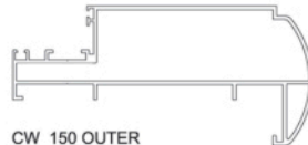
CW 150 OUTER
